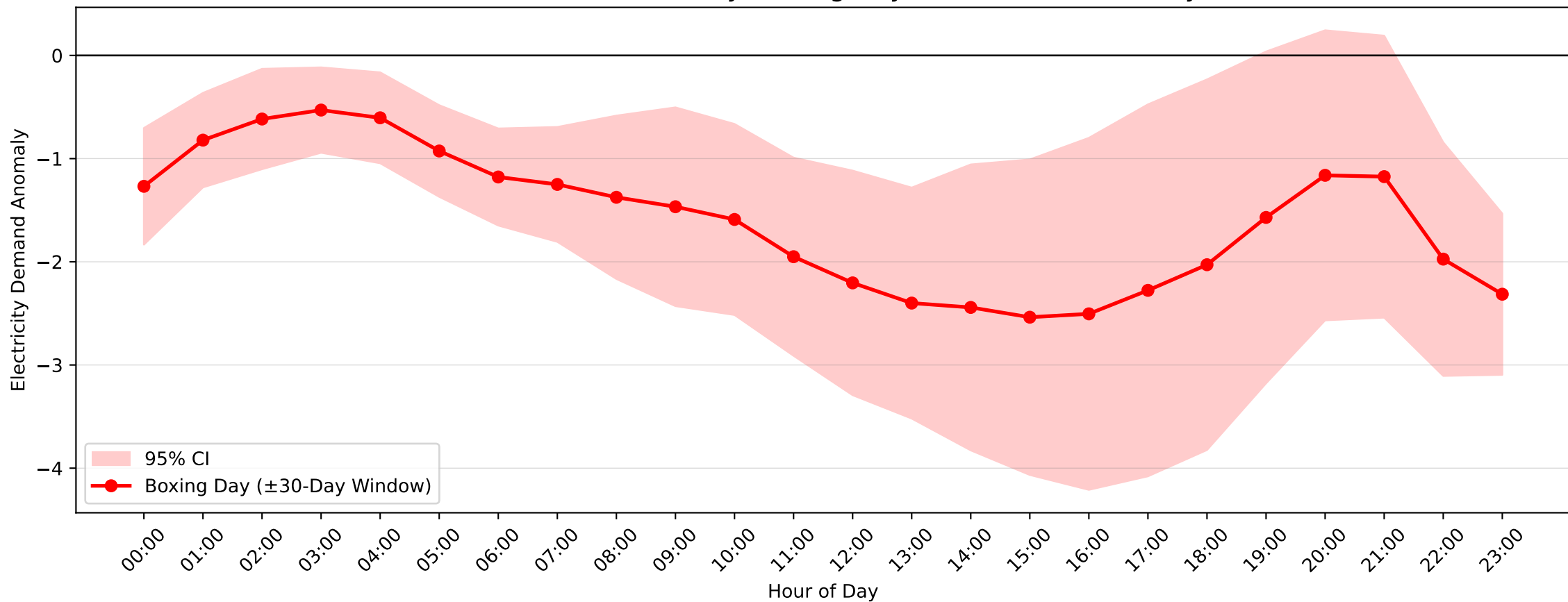
Muswellbrook Demand Anomaly: Boxing Day (2004–2017, \pm 30 -Day Window)
